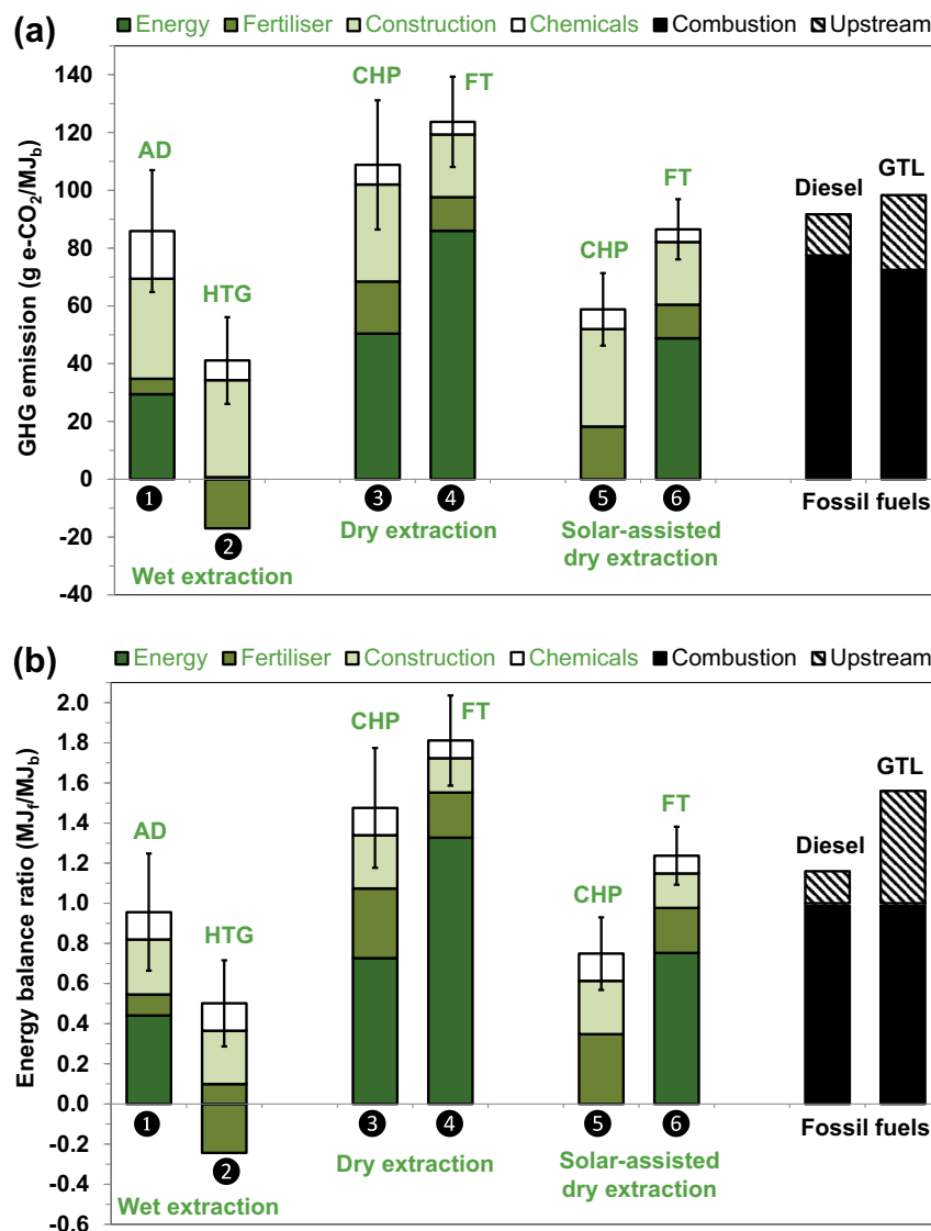
Fig. 4. Baseline values for GHG emission (a), and energy balance ratio (b) of biodiesel produced from the processes considered in this study. The corresponding values for petroleum diesel and FT diesel from natural gas (GTL) are included for comparison.
