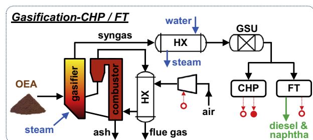
Fig. 3. Schematic process flow diagram of gasification–CHP and gasification–FT processes considered for the conversion of dry extraction OEA. Open and filled circles represent electrical and thermal energy, respectively.
