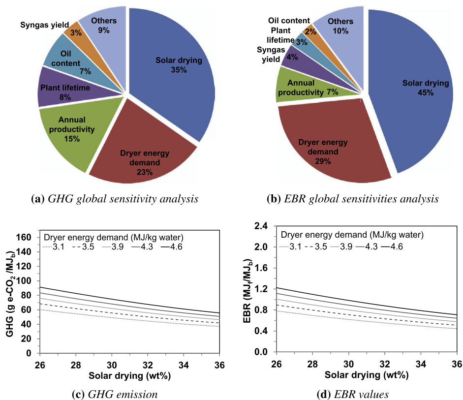
Fig. 9. Global sensitivity analysis for GHG (a), and EBR (b); and effects of the two most influencing parameters on GHG (c) and EBR (d) for solar-assisted dry extraction and integrated gasification–CHP (route 5).
