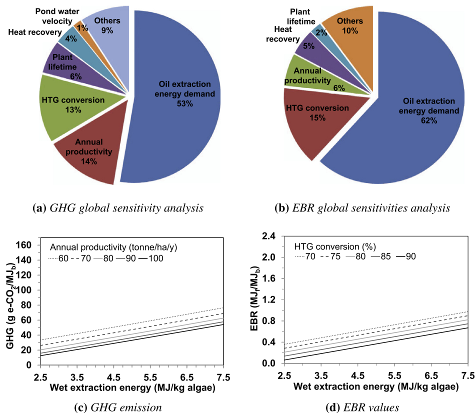
Fig. 6. Global sensitivity analysis for GHG (a), and EBR (b); and effects of the two most influencing parameters on GHG (c) and EBR (d) for the wet extraction and hydrothermal gasification (HTG) (route 2).
