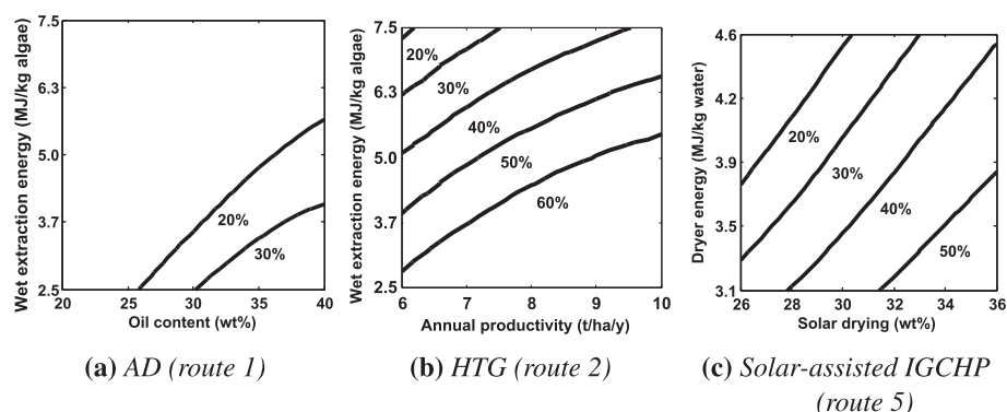
Fig. 11. Contour plots of algal biodiesel GHG reduction produced via different conversion strategies with respect to the emissions from fossil diesel.
