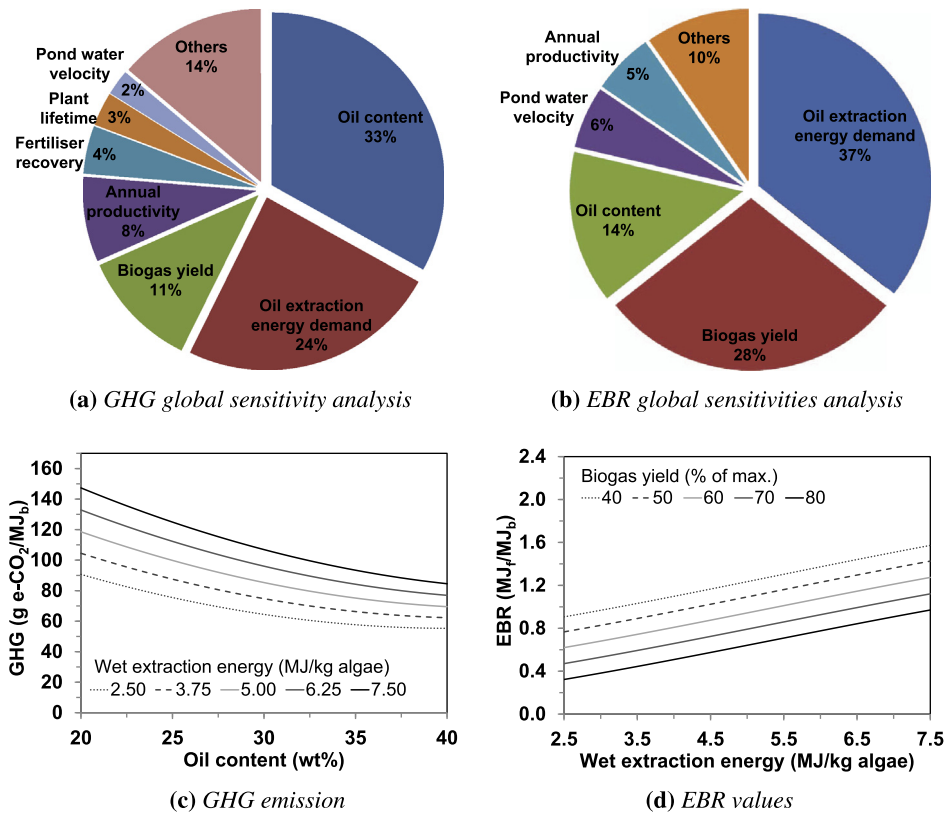
Fig. 5. Global sensitivity analysis for GHG (a), and EBR (b); and effects of the two most influencing parameters on GHG (c) and EBR (d) for biodiesel production from wet extraction and anaerobic digestion (AD) (route 1).
