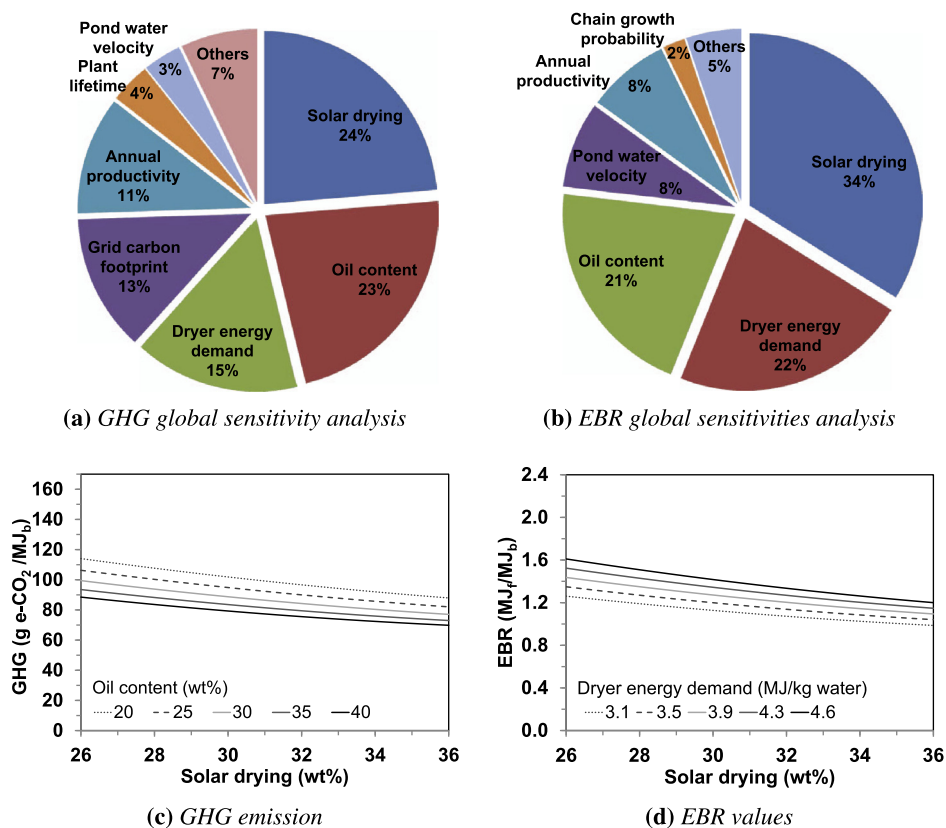
Fig. 10. Global sensitivity analysis for GHG (a), and EBR (b); and effects of the two most influencing parameters on GHG (c) and EBR (d) for solar-assisted dry extraction and integrated gasification–FT (route 6).
