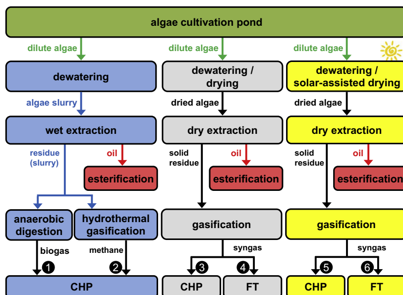
Fig. 1. Schematic process flow diagram of algal biodiesel production via wet extraction, dry extraction, and solar-assisted dry extraction with different strategies with respect to the conversion of the oil-extracted solid.
