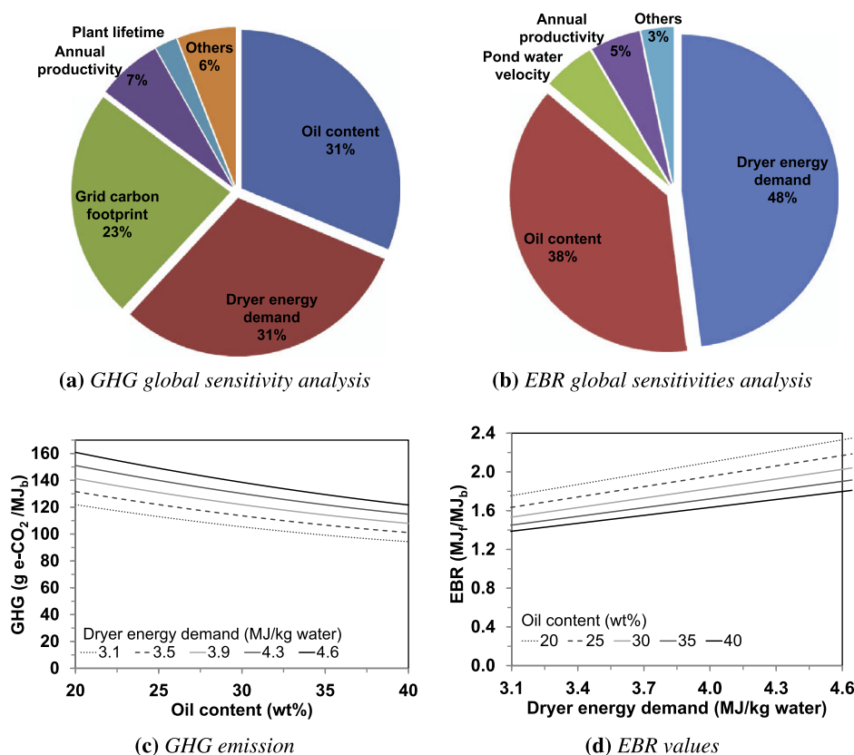
Fig. 8. Global sensitivity analysis for GHG (a), and EBR (b); and effects of the two most influencing parameters on GHG (c) and EBR (d) for dry extraction and integrated gasification–FT (route 4).
