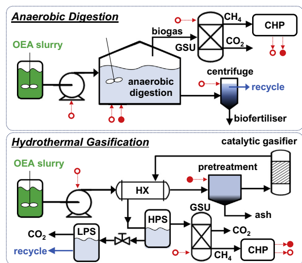
Fig. 2. Schematic process flow diagram of anaerobic digestion and hydrothermal gasification processes considered for the conversion of wet extraction OEA slurry. Open and filled circles represent electrical and thermal energy, respectively.
